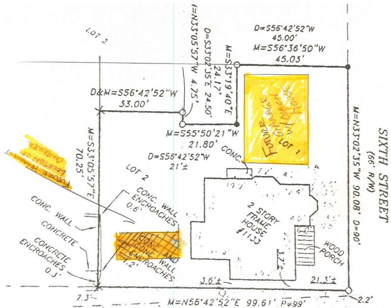
Proposed site plan noting location of shipping container in relation to the house and the street.
